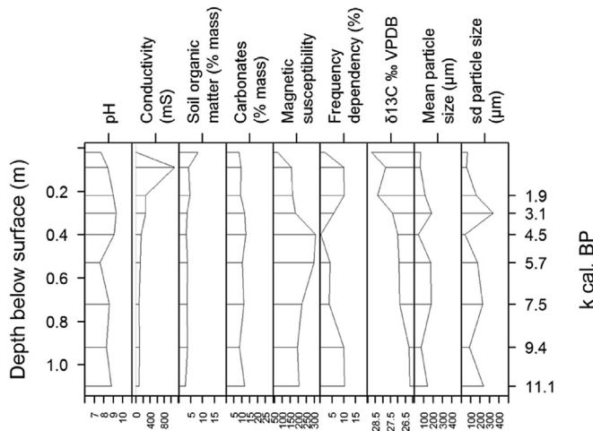
Fig. 6. Summary of bulk sediment analysis of samples from Khao Toh Chong. Magnetic susceptibility is reported as low frequency mass specific units 10^8 \text{ m}^3 \text{ kg}^{-1} . Right side axis shows modeled ages at sample location depths.
