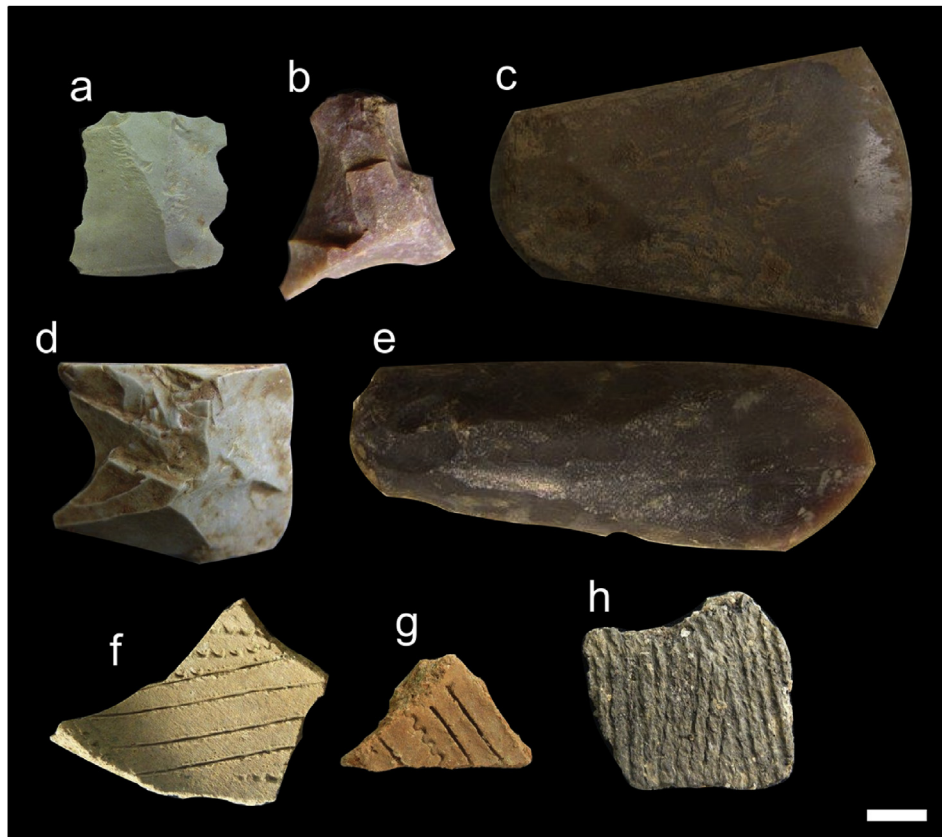
Fig. 8. Examples of ceramics, ground and flaked stone artefacts from Khao Toh Chong. a) chert flake (Excavation Unit (EU) 19), b) quartzite flake (EU18), c) quartzite polished adze (EU5), d) chert flake (EU18), e) quartzite polished adze (EU5), f & g) ceramic sherd with incised and infilled decoration (EU3), h) cord-marked ceramic (EU4).
