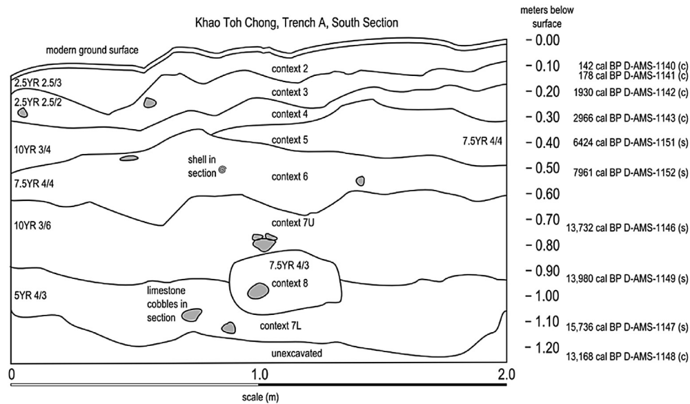
Fig. 2. South section of Khao Toh Chong rockshelter trench A. The radiocarbon ages are the midpoints of the 95% calibrated age intervals. (c) indicates charcoal and (s) indicates shell as the material dated.
