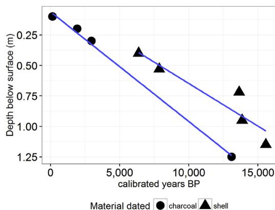
Fig. 4. Depth-age plot of calibrated radiocarbon dates from archaeological excavations at Khao Toh Chong.
