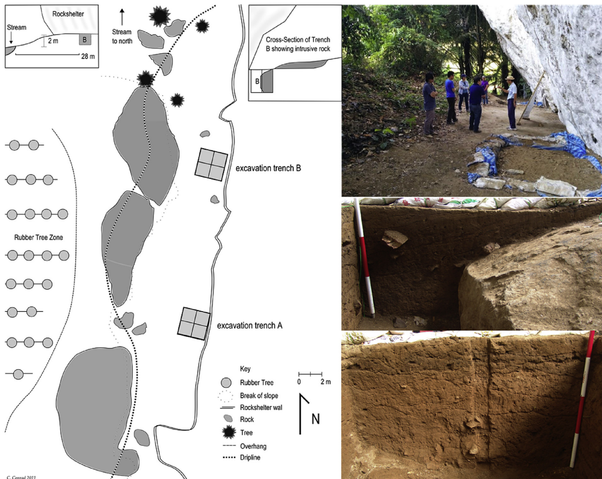
Fig. 3. Plan of Khao Toh Chong rockshelter. The top image shows a view looking North, with trench A in the foreground. The middle image shows the South section of trench B. The bottom image shows the South section of trench A.
