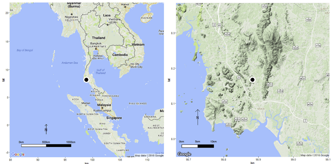
Fig. 1. Maps of the region and local area of the Khao Toh Chong rockshelter. The majority of the landscape between the site and the coast is < 30 m above the current sea level. Map data are from Google and DigitalGlobe, via ggmap (Kahle and Wickham, 2013).
