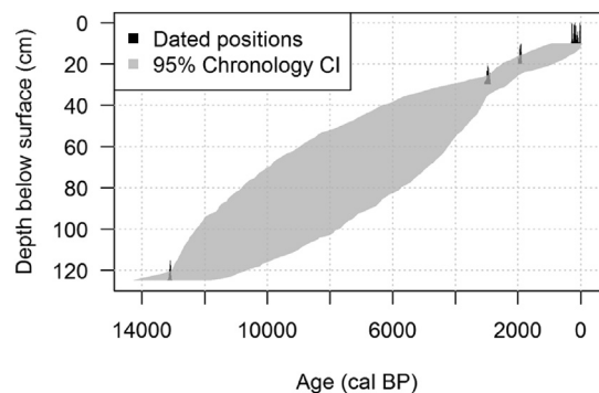
Fig. 5. Depth-age model of calibrated radiocarbon dates on charcoal from Khao Toh Chong. The grey shaded area indicates the 95% confidence interval of the age at a given depth, computed by a non-parametric chronology model fitted to age/depth data according to the Compound Poisson-Gamma model of Haslett and Parnell (2008). The black areas show the distribution of the calibrated ages.
