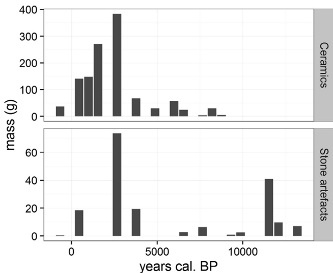
Fig. 9. Distribution of ceramics and stone artefacts in each excavation unit over time at Khao Toh Chong. Ages older than 13,000 cal BP have been extrapolated using the age-depth model described above.
