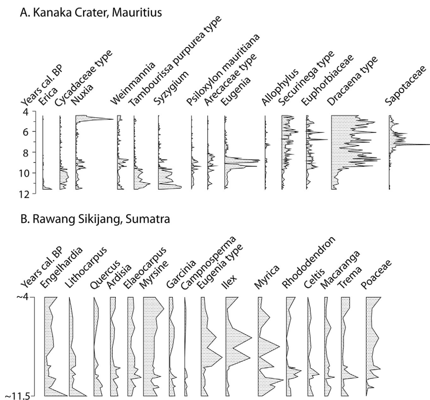
Fig. 2. Typical early Holocene pollen diagrams. A., Kanaka Crater, Mauritius, showing a clear early Holocene succession, with a sequence of taxa dominating the vegetation (after de Boer et al., 2013). B., Rawang Sikijang, Sumatra, with a disrupted succession with the disturbance indicators Celtis , Macaranga , Trema and Poaceae common from the base of the Holocene and expanding ~8 ka BP (after Flenley and Butler, 2001).
